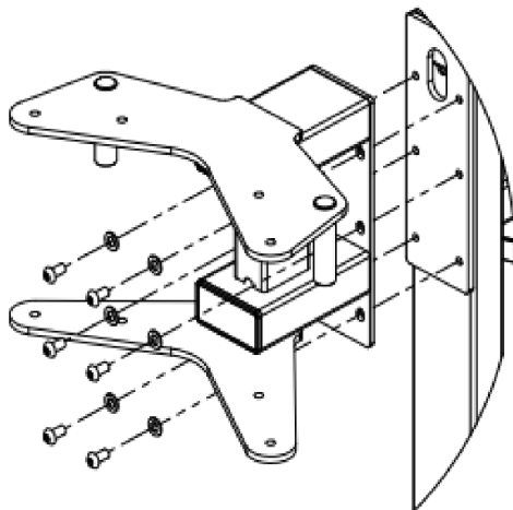
Detail View A Scale 2:5
